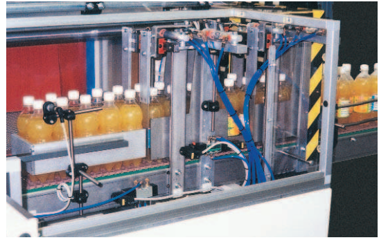
Quick feeding with partition on more rows. Output up to 15 packages/minute.
