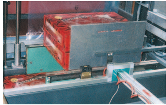
Feeding with piling up group, to get multistratus packages.
